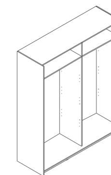
AR9340K
